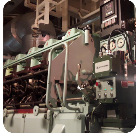
Hyundai Himsen H21/32
